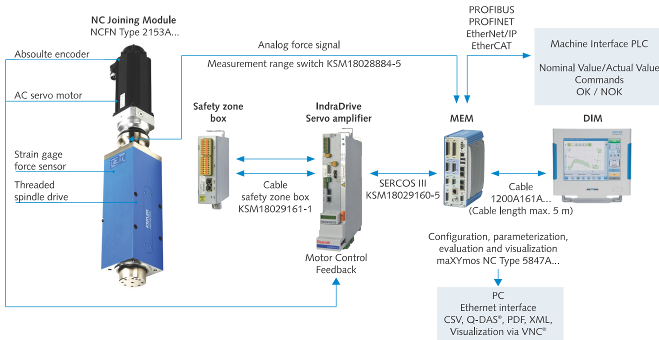
Fig. 2: Functional principle of NC joining system with NC joining module NCFN Type 2153A... and maXYmos NC Typ 5847A...
