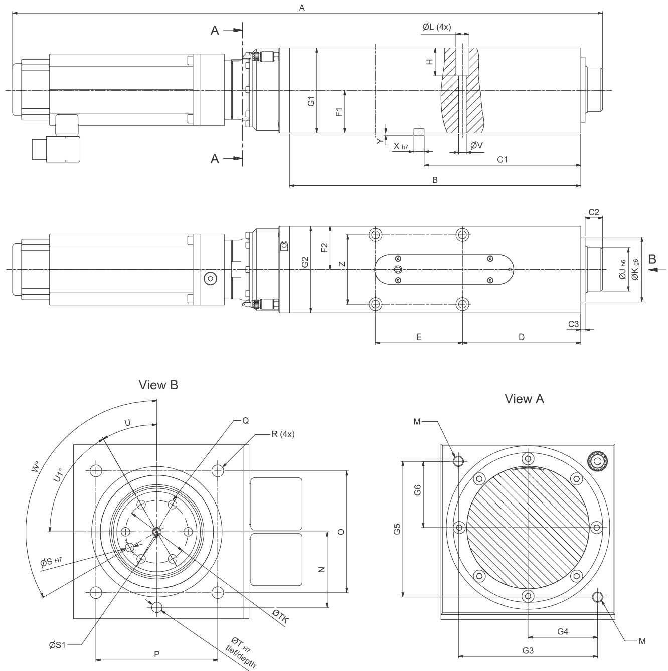
Fig. 1: Dimensions NC joining module NCFN Type 2153A...
