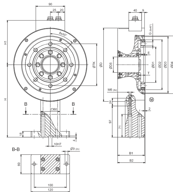
Fig. 2: Type 4510B... size 2, 500 N·m and 1 000 N·m
