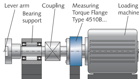
Fig. 8: Calibration facility
