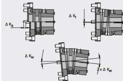
Permitted Shaft Displacements for Coupling Elements
